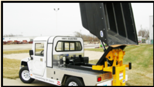
2 cubic yd. Refuse box in raised position for emptying collections.
